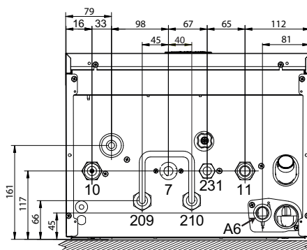
fig. 60- Bottom view
