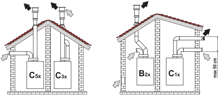
fig. 33- Examples of connection with separate pipes (⇨ = Air / ⇨ = Fumes)
